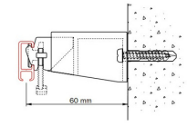
Wall mounting with 7451.
