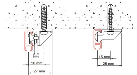
Ceiling mounting with 7450
