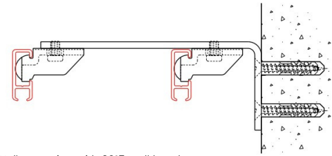
Wall mounting with 2015 wall brackets
