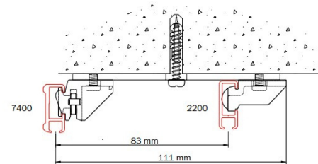
Ceiling mounting with 2216 & 7450 resp. 2250.
